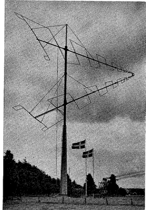
R&S® AK 226/441 Rotatable Logarithmic Periodic Antenna up to 200 kW
