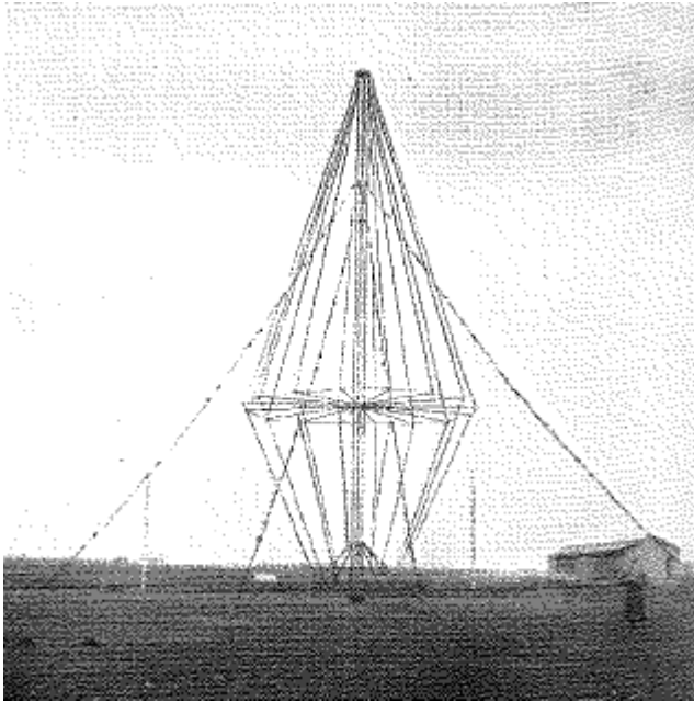
R&S® 3.6 to 26 MHz Cone Antenna up to 20 kW
