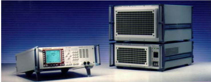
R&S® XK2100/XK2500/2900 150 / 500 / 1000W HF Transceiver Family
